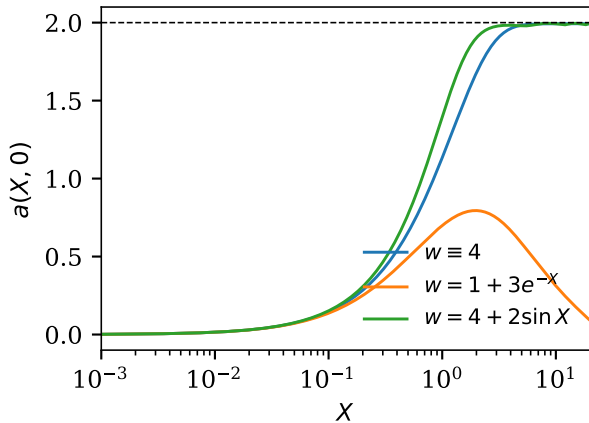
three strains, h = 1/100
