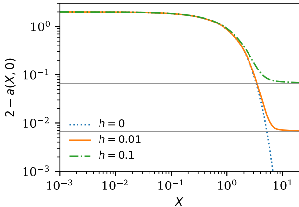
w \equiv 4 : the margin against 2h/(w - 1)
